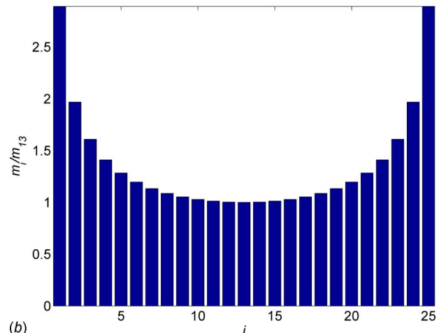
Fig. 4 Stiffness and mass elements for a 25DOF MFSG
